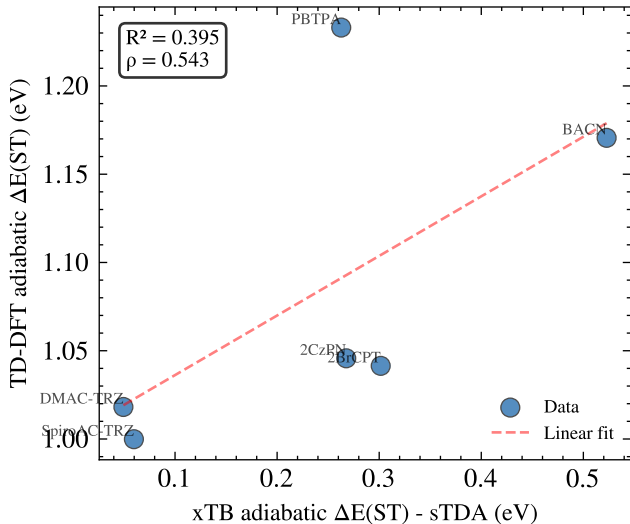
(a) sTDA method
