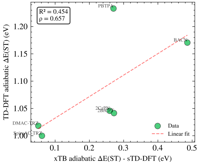
(b) sTD-DFT method
